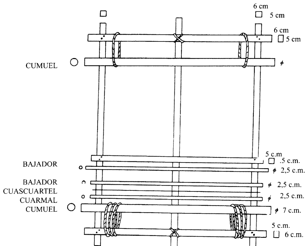
Telar vertical
